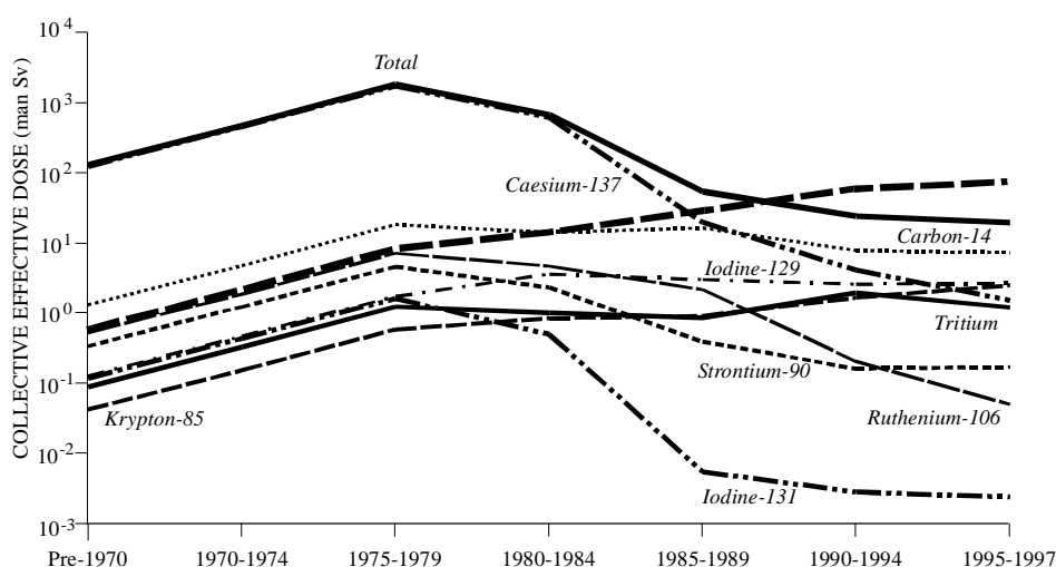
Figure XX. Local and regional collective effective doses from average annual release of radionuclides from fuel reprocessing plants. The amount of fuel reprocessed is indicated by the heavy dashed line (units GW a).
