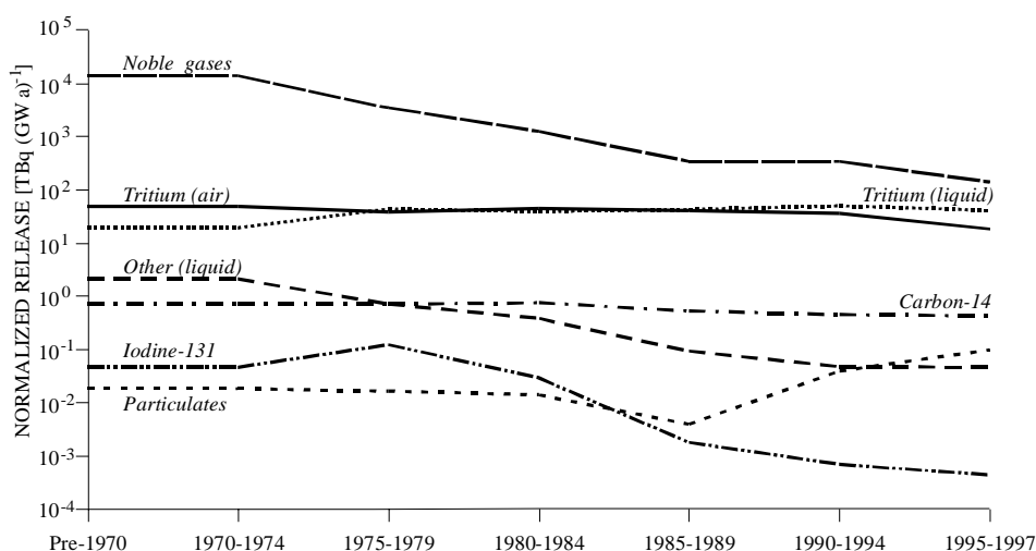
Figure XVII. Trends in releases of radionuclides from reactors.
