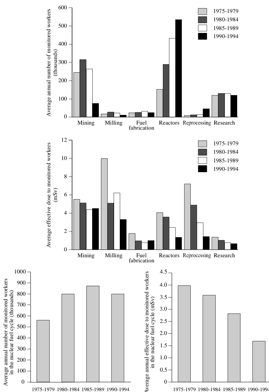
Figure VI. Trends in numbers of monitored workers and doses to workers in the nuclear fuel cycle.
